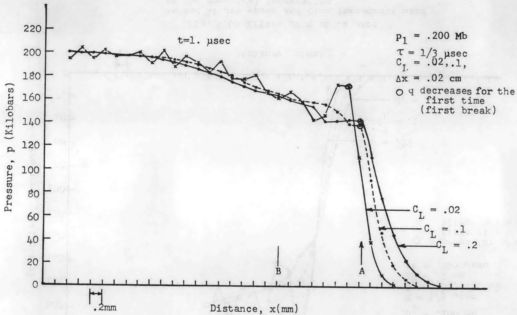
Fig.5.11r-Effect of q at 1. \mu\text{sec} . \Delta x and \Delta t are space and time increments used in the numerical integration.
