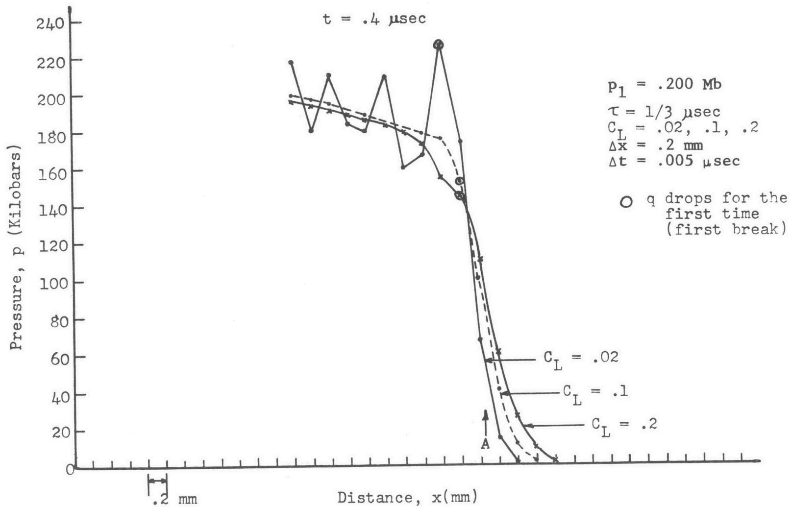
Fig. 5.10—Effect of q at .4 \mu\text{sec} . \Delta x and \Delta t are space and time increments used in the numerical integration.
